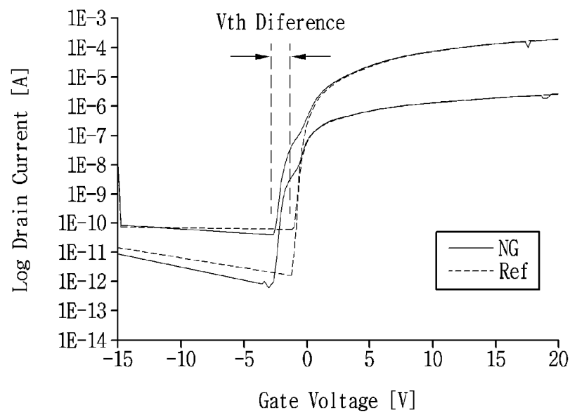
FIG. 1 (Related Art)
