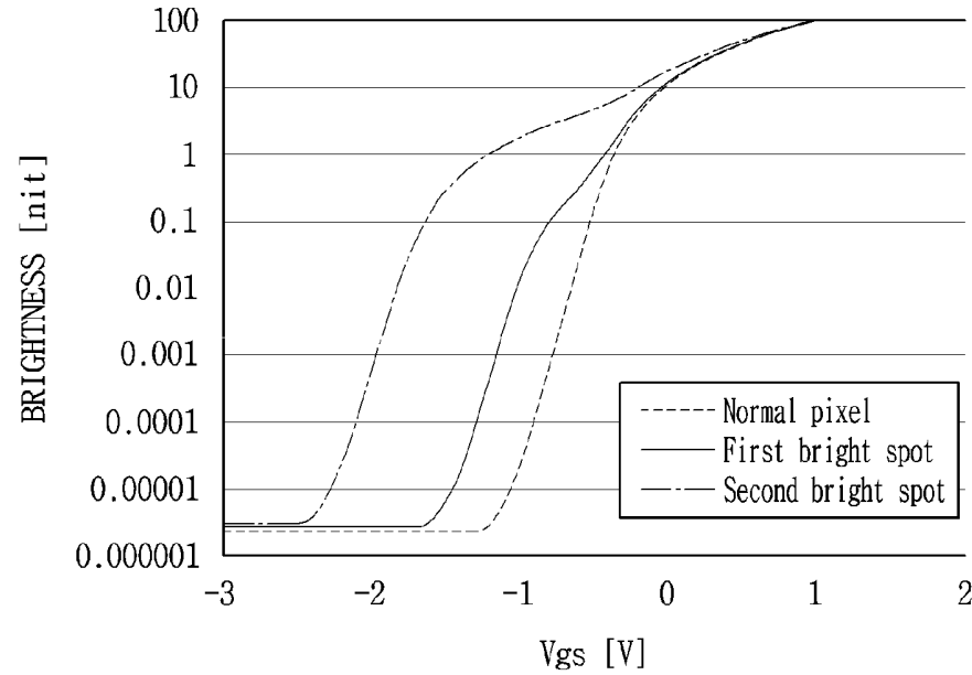
FIG. 2 (Related Art)
